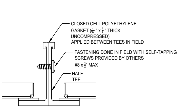
A HALF TEE FIELD JOINT
