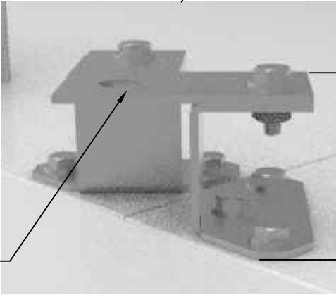
TWO MODULE CORNER BRACE DETAIL
