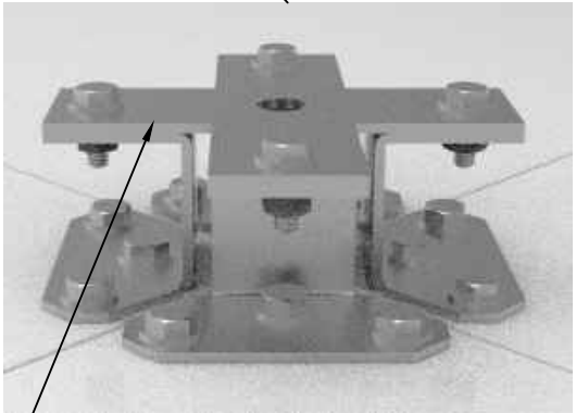
FOUR MODULE CENTER BRACE DETAIL
