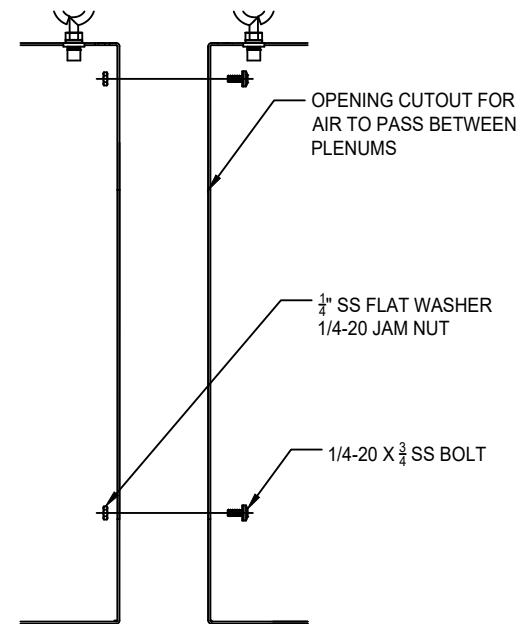
E BOLTED JOINT ASSEMBLY
