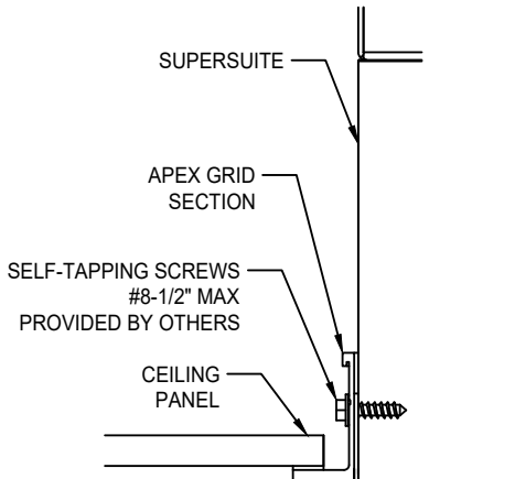
C APEX GRID INTEGRATION
